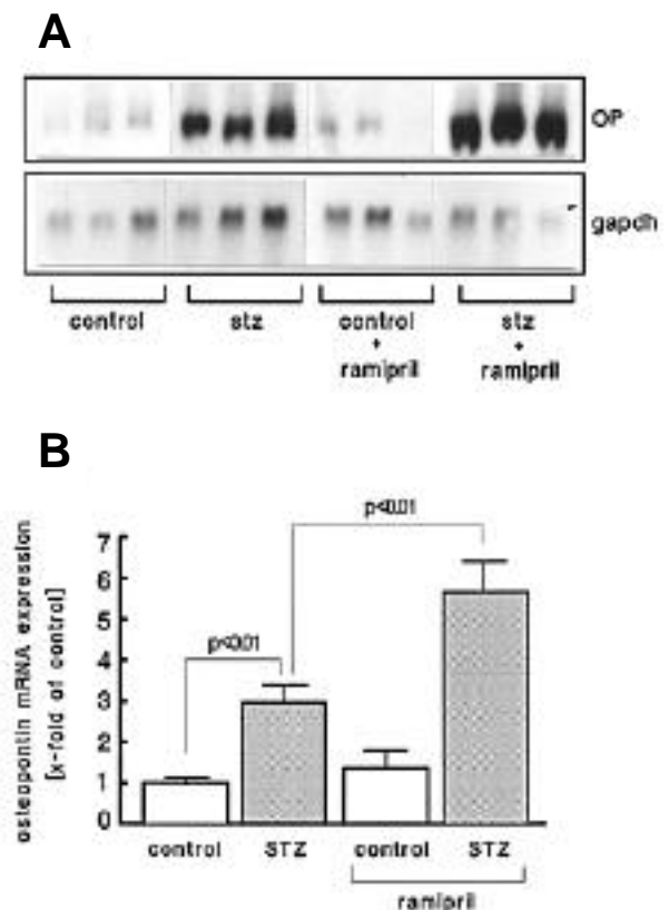
FIG. 2. Effect of ramipril treatment on renal cortical osteopontin expression in normal and diabetic rats at 12 weeks. Figure shows the Northern blot analysis of cortical extracts from normal and diabetic (STZ) rats treated with ramipril (3 mg · kg -1 · day -1 ) (A). In addition to osteopontin, membranes were probed with GAPDH. Quantitative analysis of Northern blots by densitometry (B). Values are corrected for RNA loading using the GAPDH signals and expressed as fold difference compared to controls ( n = 6, mean ± SE).
