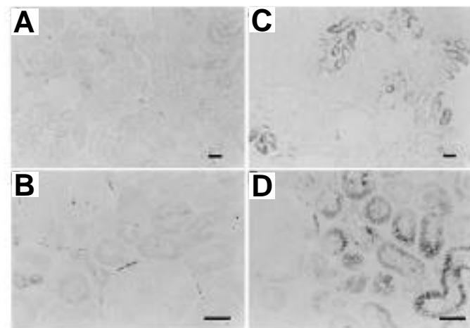
FIG. 4. Osteopontin protein expression in renal cortices of nondiabetic ( A, B ) and STZ-diabetic ( C, D ) rats after treatment (12 weeks) with ramipril. Immunostaining was performed with the anti-osteopontin antibody OP199. No staining was observed when a nonimmune antibody was used as control (not shown). Size bar = 150 \mu\text{m} .
