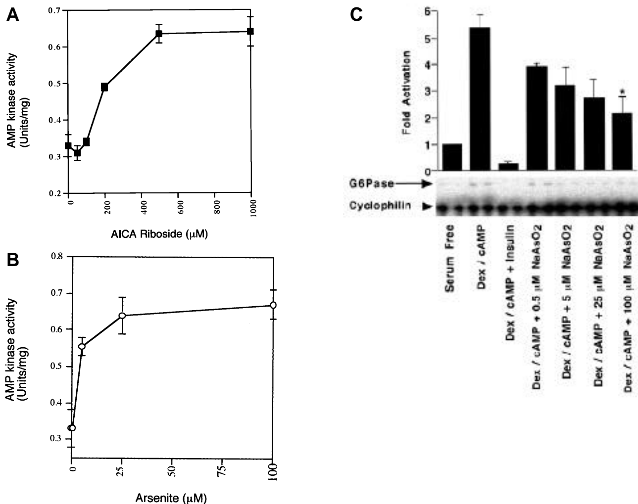
FIG. 4. The effects of AICAR and sodium arsenite on gene expression correlate with activation of AMPK. H4IIE cells were serum starved overnight before a 5-min incubation with AICAR ( A ) or a 3-h incubation with sodium arsenite ( B and C ) at the concentrations indicated. Cell lysates were prepared and the activity of AMPK was measured ( A and B ), or total RNA was isolated and G6Pase mRNA was determined ( C ) as described in RESEARCH DESIGN AND METHODS. Results are the average \pm SE of 2 experiments carried out in duplicate (* P < 0.01 ).
