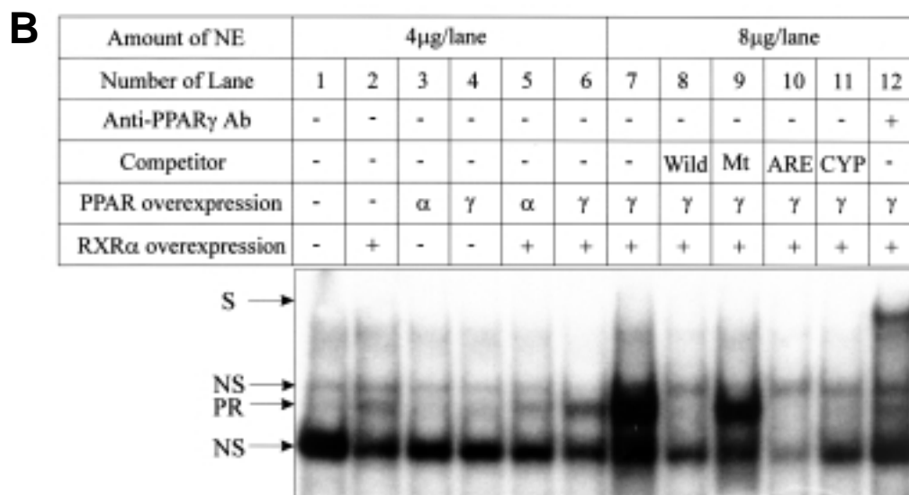
FIG. 4. A: Sequence comparison of PPREs from various genes. Sequences of GLUT2-PPRE and its mutant form GLUT2-PPREmt, ARE (23), and CYP (24) are compared with the consensus sequence of PPRE. PPRE sequence is underlined, and mutated bases are lowercase (28). B: EMSA of GLUT2-PPRE. The ^{32} P-labeled double-strand oligonucleotide GLUT2-PPRE was incubated with nuclear extracts (4 or 8 µg) from CV-1 cells transfected with expression vectors of PPARs and/or RXR- \alpha as indicated. For competition experiments, 50 mol/l excess of GLUT2-PPRE (Wild), GLUT2-PPREmt (Mt), ARE, and CYP were included in the binding reaction. For the supershift experiment, 1 µg anti-PPAR- \gamma antibody was used. PR indicates the shifted band by heterodimer of PPAR/RXR- \alpha , and S indicates the supershifted band by anti-PPAR- \gamma antibody. Ab, antibody; DR+1, the hexamer sequence AGGTCA in a direct repeat formation spaced by 1 nucleotide; NE, nuclear extract; NS, nonspecific binding; PR, binding of PPAR/RXR- \alpha heterodimer; S, supershifted band.
