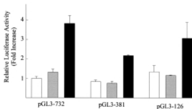
FIG. 2. Identification of the PPRE in the promoter region of the rat GLUT2 gene. Luciferase reporter constructs under the control of the rat GLUT2 promoter, each spanning from -732, -381, and -126 to +189, were cotransfected into CV-1 cells with or without PPARs and RXR- \alpha expression vectors. The cells were incubated in the presence or absence of respective ligands as indicated. A total of 10 \mu mol/l WY14643 for PPAR- \alpha , 10 \mu mol/l troglitazone for PPAR- \gamma , and 1 \mu mol/l 9- cis retinoic acid for RXR- \alpha was used as ligand. Normalized luciferase activities are shown as means \pm SE of 3 independent experiments in triplicate and are expressed as the fold-increase relative to the basal activity of pGL3-732 in the absence of expression vectors and ligands. \square , Control; \blacksquare , PPAR- \alpha /RXR- \alpha (vehicle, WY14643/9- cis retinoic acid); \blacksquare , PPAR- \gamma /RXR- \alpha (vehicle, troglitazone/9- cis retinoic acid).
