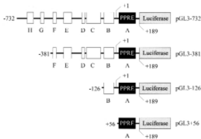
FIG. 1. Structure of the rat GLUT2 promoter. Boxes represent the protein binding sites reported by Kim and Ahn (27). Site A indicates the region containing a possible PPRE; +1 represents the transcription initiation site.
