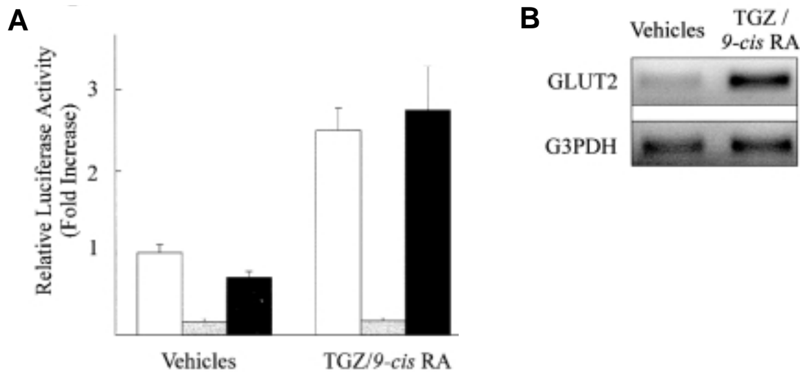
FIG. 5. A: Activation of the rat GLUT2 promoter by endogenous PPAR- \gamma and RXR- \alpha in HIT-T15 cells. HIT-T15 cells were transfected with pGL3-732 (□), pGL3-732m (▣), or PPRE3-tk-LUC (■). The cells were then treated with 20 \mu M troglitazone (TGZ) and 2 \mu M 9- cis retinoic acid (RA) or their vehicles. The PPRE3-tk-LUC reporter was constructed by inserting 3 copies of an oligonucleotide encoding the PPRE (GTCTGA CAGGGGACCAGGACAAAAGGTACGTTCCGGGAGTCGAC) in direct orientation to the unique Sa I site of the basal reporter construct tk-LUC (16). Normalized luciferase activities are shown as means \pm SE of 3 independent experiments in triplicate and are expressed as the fold-increase relative to the basal activity of pGL3-732 in the absence of ligands. B: Effect of troglitazone and 9- cis retinoic acid on GLUT2 expression in the isolated primary islets of rats. Isolated primary islets were incubated for 3 days in the presence or absence of 20 \mu M troglitazone and 2 \mu M 9- cis retinoic acid, and total RNA was prepared. RT-PCR was adapted to measure the GLUT2 mRNA semiquantitatively. Quantitation of PCR products was performed by densitometric scanning using Molecular Analyst (Bio-Rad), and quantity of GLUT2 mRNA was normalized with respect to G3PDH mRNA.
