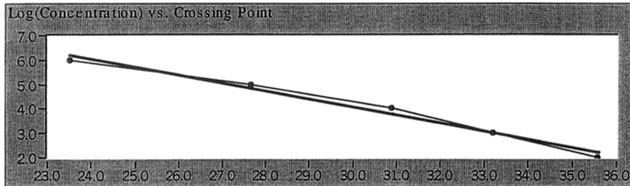
FIG. 2. Quantitation of PCR products. A : Logarithmic plot of fluorescence versus cycle number of perforin of rhesus monkey. B : Standard curve constructed with the perforin standards from 10^6 to 10^2 copies. The standard curve was constructed by plotting the logarithmic concentration of the standard versus the crossing points (cycle number). The error of the standard curve ( \epsilon ) = 3.4353E-3 ( \epsilon = sum of squares of deviation/number of measuring points).
