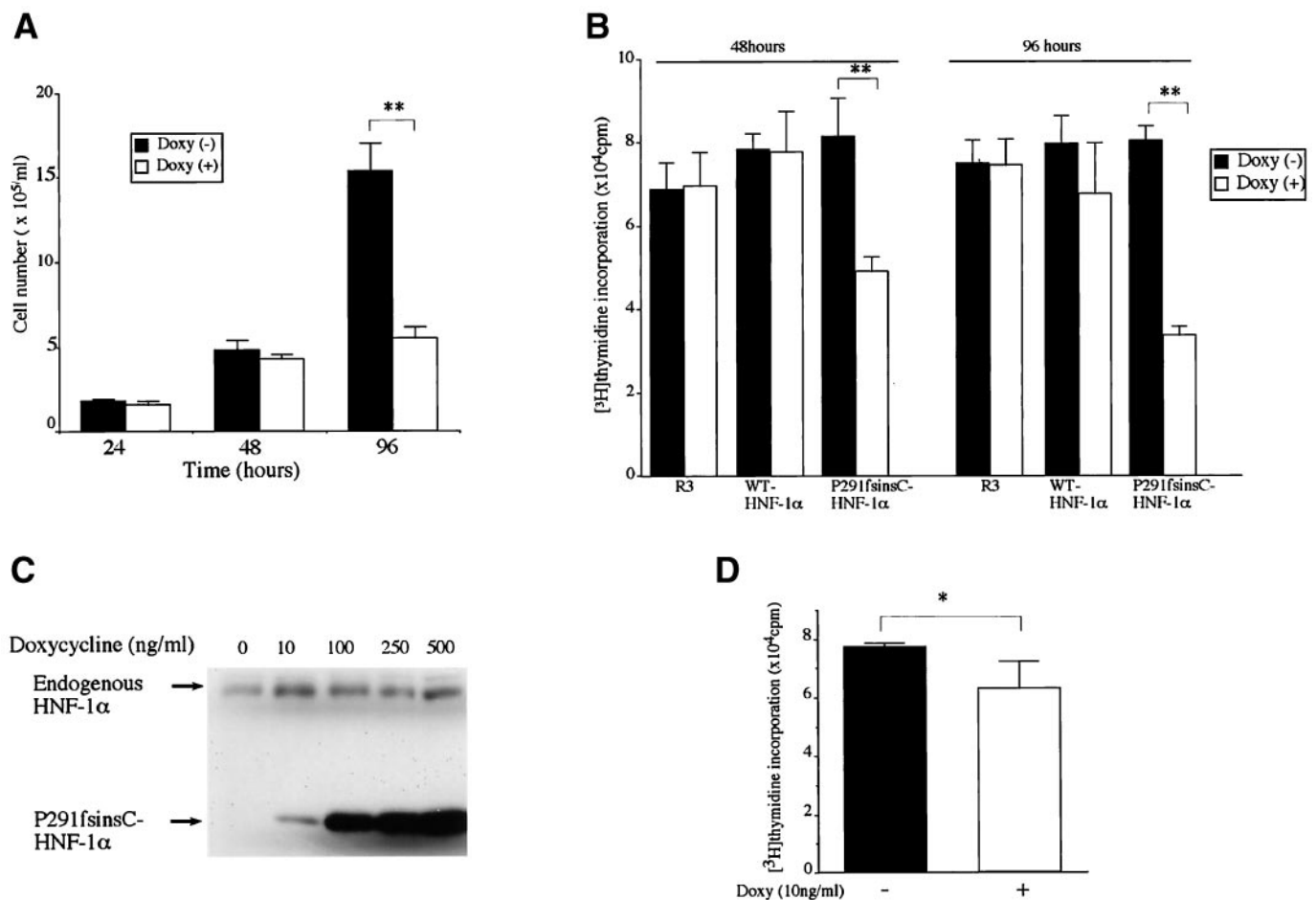
FIG. 1. Effects of P291fsinsC-HNF-1 \alpha on cell growth. A: Number of HNF-1 \alpha -P291fsinsC#32 INS-1 cells cultured with or without 500 ng/ml doxycycline (Doxy) for 24, 48, or 96 h. Data are means \pm SE of five independent counts. ** P < 0.001. B: [ 3 H]thymidine incorporation in induced and noninduced INS-r3, HNF-1 \alpha #15, and HNF-1 \alpha -P291fsinsC#32 cells for 48 or 96 h. Data are means \pm SE of three independent experiments performed in triplicate. ** P < 0.001. C: Expression of endogenous HNF-1 \alpha and P291fsinsC-HNF-1 \alpha in HNF-1 \alpha -P291fsinsC#32 cells cultured with different concentrations of doxycycline for 48 h. D: [ 3 H]thymidine incorporation of HNF-1 \alpha -P291fsinsC#32 cells cultured with or without 10 ng/ml doxycycline for 48 h. Data are means \pm SE of three experiments performed in triplicate. * P < 0.01.
