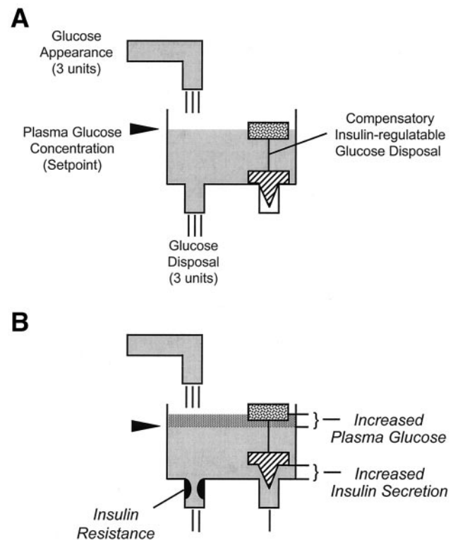
FIG. 4. Schematic representation of the feed-forward system: insulin resistance \rightarrow increased glycemia \rightarrow increased insulin secretion. At steady state, glucose appearance equals glucose disposal and glucose concentration remains unchanged. A fixed glucose concentration (liquid level) is assumed, representing the set stimulus for a given insulin secretion (level of the floating plug). A : Representing the normal state, the compensatory insulin-regulatory glucose disposal is not activated (closed plug). B : The “normal,” fully compensated insulin-resistant state. Decreased glucose disposal results in an increased glucose concentration that in turn will cause the “floating plug” to rise (increased insulin secretion) and permit compensatory glucose disposal. This rise will continue until the total glucose disposal again equals glucose appearance. To secure continuous patency of the compensatory outlet, the glucose level must stay above the original set point level. A (theoretical) replugging of the compensatory outlet would instantaneously cause an increase in glucose concentration and therefore cannot happen as long as the obstruction due to insulin resistance is present.
