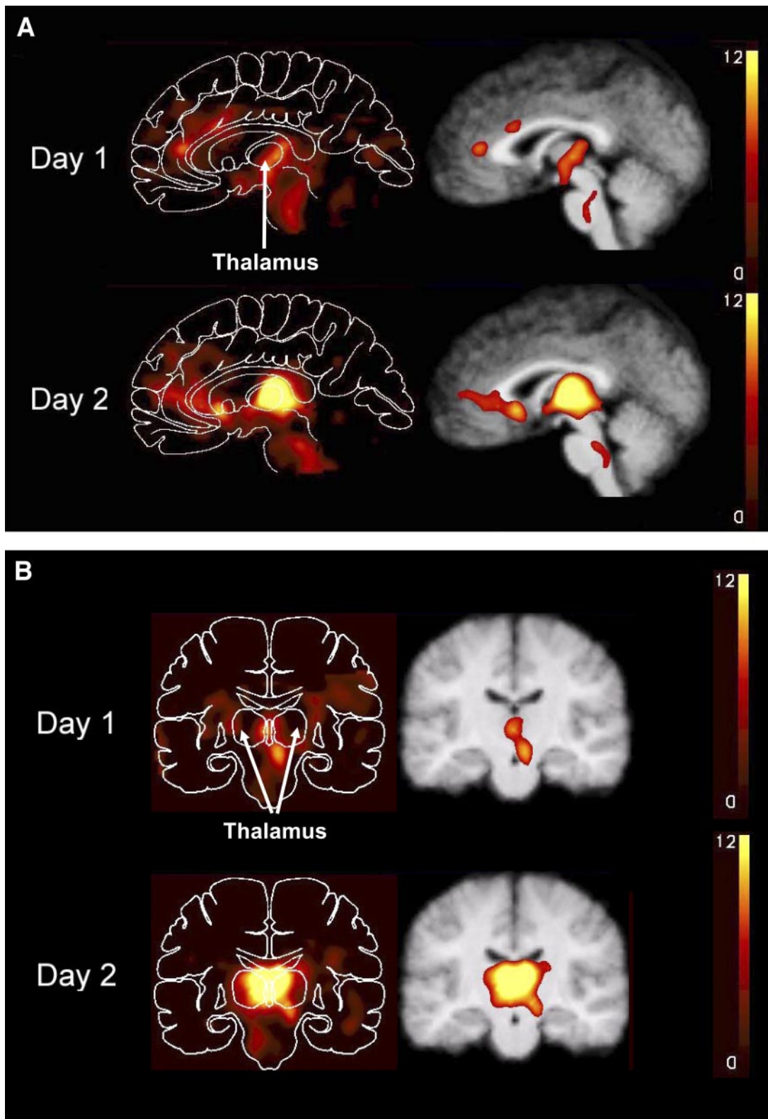
FIG. 1. Regional cerebral blood flow changes during hypoglycemia illustrating greater synaptic activity in bilateral dorsal midline thalamus on day 2, following ~24 h of interval interprandial hypoglycemia, compared with day 1. These are combined subtraction images from all PET scans from all nine subjects superimposed on the combined MR image. The color scales show changes relative to mean global blood flow. A maximum of 12% is used for all scales. However, the maximum change for day 2 was 18% compared with 10% on day 1. A: Mid-sagittal slices. B: Coronal slices at the level of the paraventricular nuclei ( y = -19 ) with the left of the brain on the left (33).
