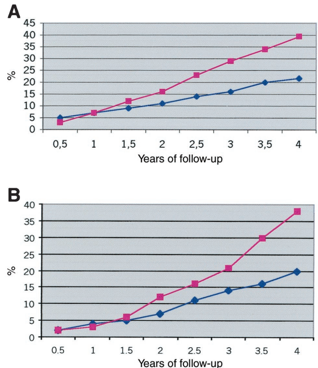
FIG. 2. Cumulative percentage of individuals in whom serum creatinine doubled from baseline (A) and of those who either died or reached ESRD (B) of CR-LIPE (◆), control (■).
