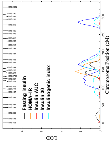
Chromosome 1
