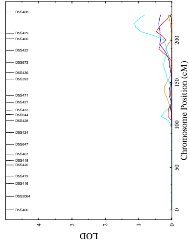
Chromosome 5
