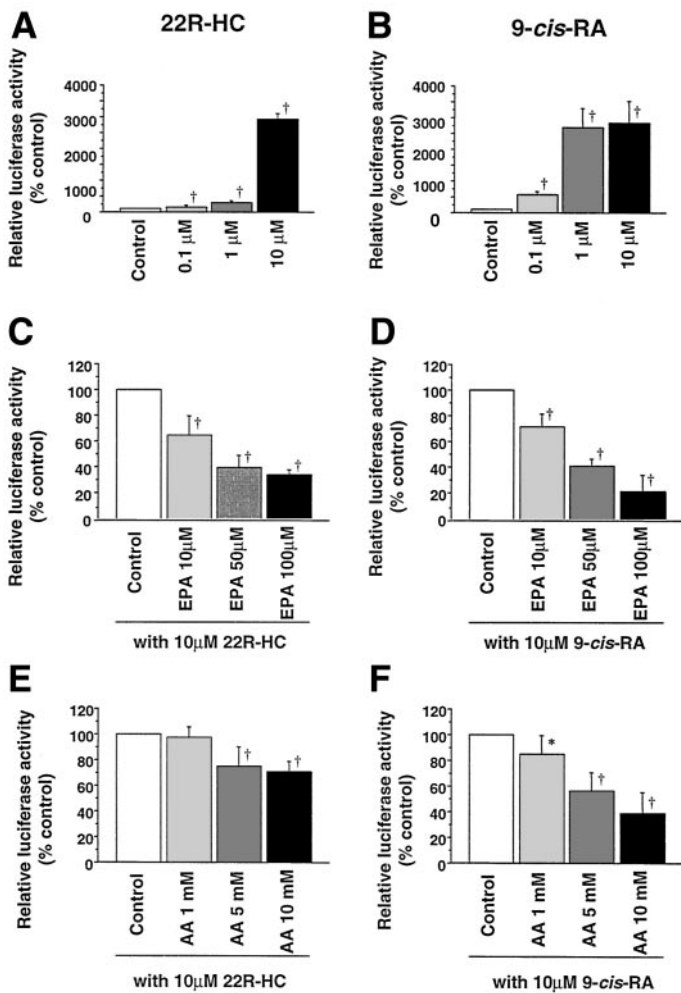
FIG. 4. Dose-dependent effects of 22( R )-hydroxycholesterol, 9- cis -RA, eicosapentaenoic acid, and acetoacetate on the activity of the human ABCA1 promoter in RAW264.7 cells. The human ABCA1 promoter was inserted into the firefly luciferase reporter gene. RAW 264.7 cells were transfected to ABCA1 gene with pGL3 basic vector together with pRL SV40 as a control reporter plasmid (renilla luciferase). After transfection, the cells were incubated with 22R-HC, 9- cis -RA, EPA, and acetoacetate (AA) for 18 h. The firefly luciferase activity was divided by the renilla activity to give a normalized value as the relative luciferase activity, and the values are shown in percent change compared with control. 22R-HC (A) and 9- cis -RA (B) dose-dependently increase the ABCA1 promoter activity. These stimulatory effects of 22R-HC (C and E) and 9- cis -RA (D and F) are dose-dependently suppressed by EPA (C and D) and acetoacetate (E and F). Results represent means \pm SD of at least four independent transfections. † P < 0.01 , * P < 0.05 compared with control (one-way ANOVA).
