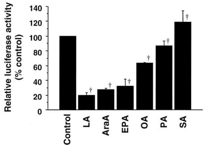
FIG. 5. The effects of various fatty acids on the activity of the human ABCA1 promoter in RAW264.7 cells. For experimental details see legend of Fig. 4. After transfection, the cells were incubated with 100 \mu mol/l EPA, oleic acid (OA), palmitic acid (PA), linoleic acid (LA), arachidonic acid (AraA), or stearic acid (SA) in the presence of 10 \mu mol/l 22R-HC and 10 g/l BSA for 18 h. Results represent means \pm SD of four independent transfection experiments. † P < 0.01 compared with control (one-way ANOVA).
