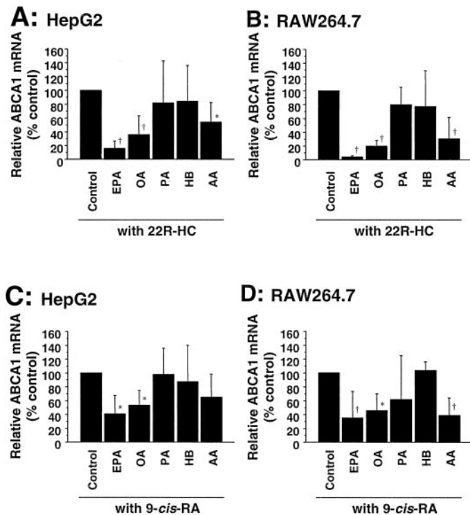
FIG. 3. Interacting effects of 22(R)-hydroxycholesterol and 9-cis-RA with fatty acids and ketone bodies on the expression of ABCA1 in HepG2 cells and RAW264.7 cells. Confluent hepatocytes (A and C) and RAW264.7 cells (B and D) were incubated for 18 h with serum-free medium in the presence of 10 g/l BSA and 10 \mu\text{mol/l} 22R-HC (A and B) or 10 \mu\text{mol/l} 9-cis-RA (C and D) plus 100 \mu\text{mol/l} EPA, 500 \mu\text{mol/l} palmitic acid (PA), 500 \mu\text{mol/l} oleic acid (OA), 10 mmol/l hydroxybutyrate (HB), or 10 mmol/l acetoacetate (AA). The mRNA of ABCA1 was demonstrated by quantitative real-time PCR. Note that EPA, oleic acid, and acetoacetate (more prominent in macrophages, but not palmitic acid and hydroxybutyrate) (B) suppress the stimulatory effect of 22(R)-HC on ABCA1 gene expression. EPA and oleic acid have less suppression on ABCA1 expression in the presence of 9-cis-RA than in 22(R)-HC. Results represent means \pm SD from four to six experiments. \dagger P < 0.01 , *P < 0.05 compared with control (one-way ANOVA).
