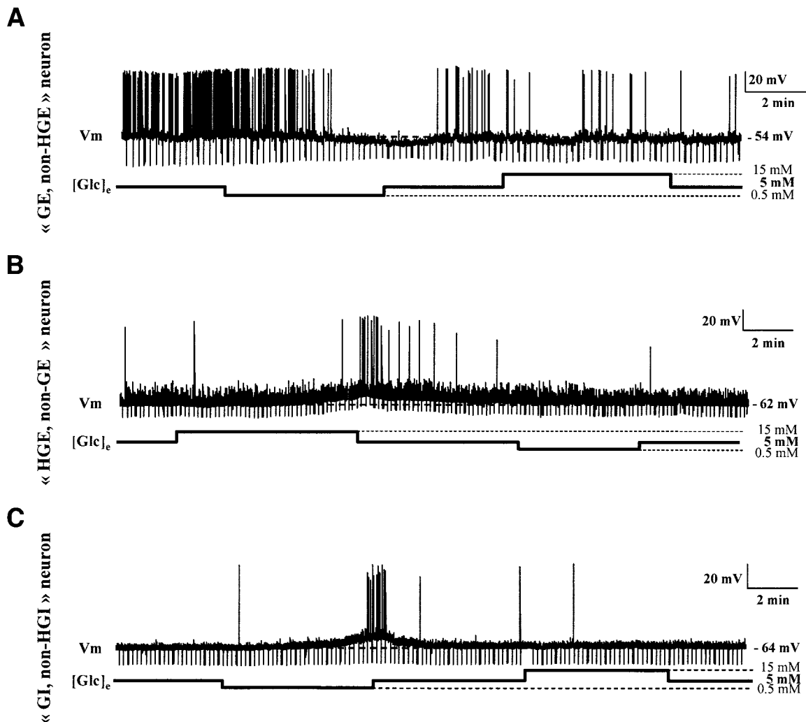
FIG. 1. Whole-cell current-clamp recordings of ARC glucosensing neurons as extracellular glucose concentration is altered. In this and all subsequent figures, downward deflections represent membrane voltage responses to hyperpolarizing current injection. Resting membrane potential is indicated by the dotted line and noted on the right . Glucose changes are schematically displayed below each recording. A: Decreased glucose inhibited this glucose-excited neuron; however, increased glucose had no effect. B: Increased glucose excited this high glucose-excited neuron; however, decreased glucose had no effect. C: Decreased glucose excited this glucose-inhibited neuron; however, increased glucose had no effect.
