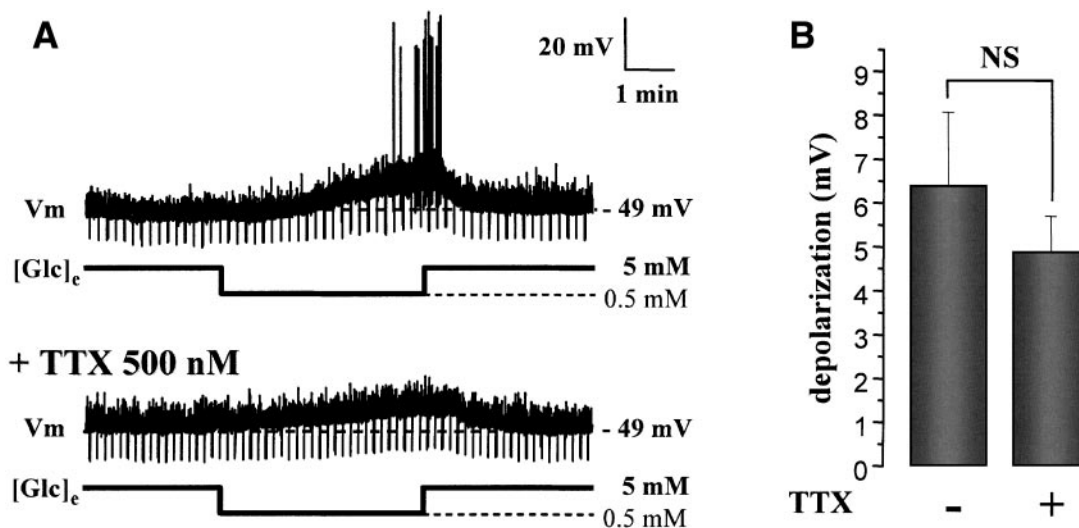
FIG. 2. A : Consecutive whole-cell current-clamp recordings in an ARC glucose-inhibited neuron. Decreased glucose excited this neuron in the presence ( bottom trace ) and absence ( top trace ) of 500 nmol/l TTX. B : The presence of 500 nmol/l TTX did not alter glucose-inhibited neurons membrane potential; n = 5 ; NS, P > 0.05 .
