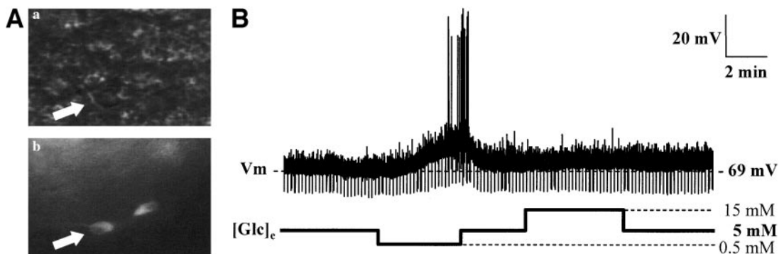
FIG. 5. A : A NPY-GFP neuron (white arrow) visualized with \times 40 objective under (a) infrared and (b) fluorescent light. B : Whole-cell current-clamp recording of an ARC NPY neuron to altered glucose concentration.
