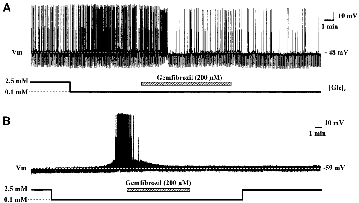
FIG. 4. Whole-cell current-clamp recordings in glucose-inhibited neurons. A : In this ARC glucose-inhibited neuron, gemfibrozil (200 μmol/l) reversed the excitatory effect of decreased glucose. This did not reverse upon washout. B : The effects of gemfibrozil were similar in this VMN glucose-inhibited neuron. After gemfibrozil washout, this neuron did not respond to changes in glucose.
