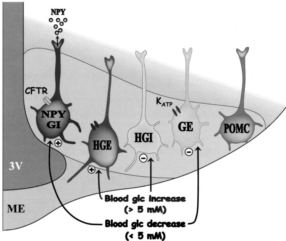
FIG. 7. ARC glucosensing mechanisms. Decreased glucose concentration <5 mmol/l in ARC inhibits glucose-excited neurons by opening the K ATP channel and excites NPY/glucose-inhibited neurons, causing NPY release by closing a CFTR-like chloride channel. Increased glucose >5 mmol/l in ARC excites high glucose-excited neurons by closing a nonselective cation channel and inhibits high glucose-inhibited neurons.
