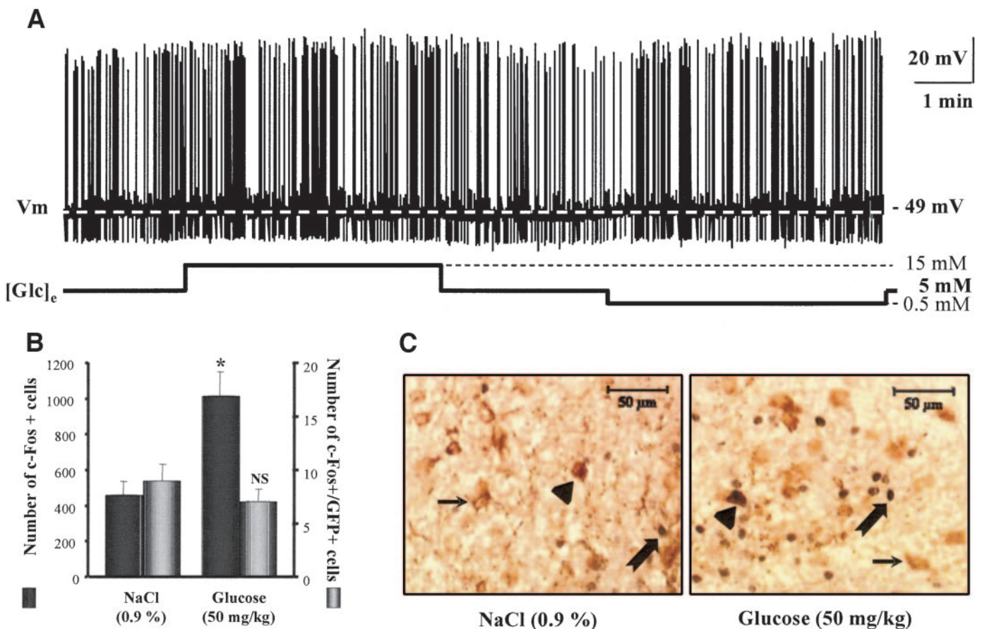
FIG. 6. A: Whole-cell current-clamp recording of an ARC POMC neuron to altered glucose concentration. Changes in glucose did not change this POMC neuron's activity. B: The mean number of c-Fos-immunopositive nuclei (left y -axis) and the number of GFP and c-Fos double immunopositive cells (right y -axis) in ARC after NaCl or glucose intracarotid injection. * P < 0.05 vs. NaCl; NS, P > 0.05 vs. NaCl. C: Illustration of GFP-immunopositive neurons (thin arrow), c-Fos-immunopositive nuclei (large arrow), and double-labeled cells (arrowhead) after intracarotid injection of NaCl (0.9%; left panel) or glucose (50 mg/kg; right panel) in POMC-GFP mice.
